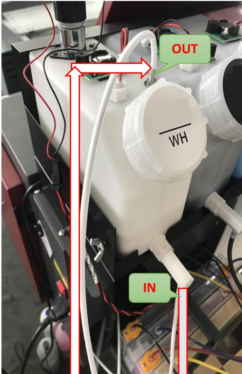
White ink circulation ink and adjustment
